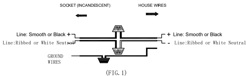
Wiring Diagram
