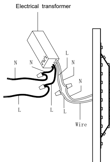
Wire connecting view
