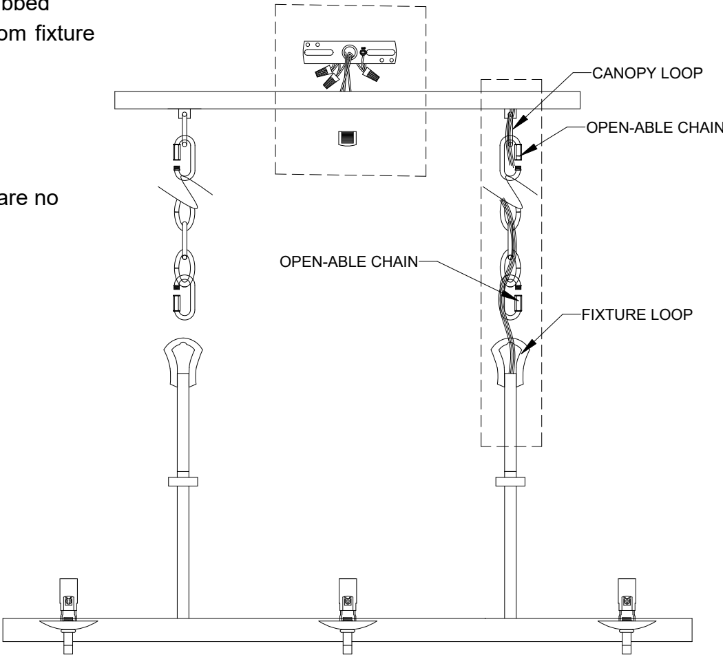
FRONT VIEW
