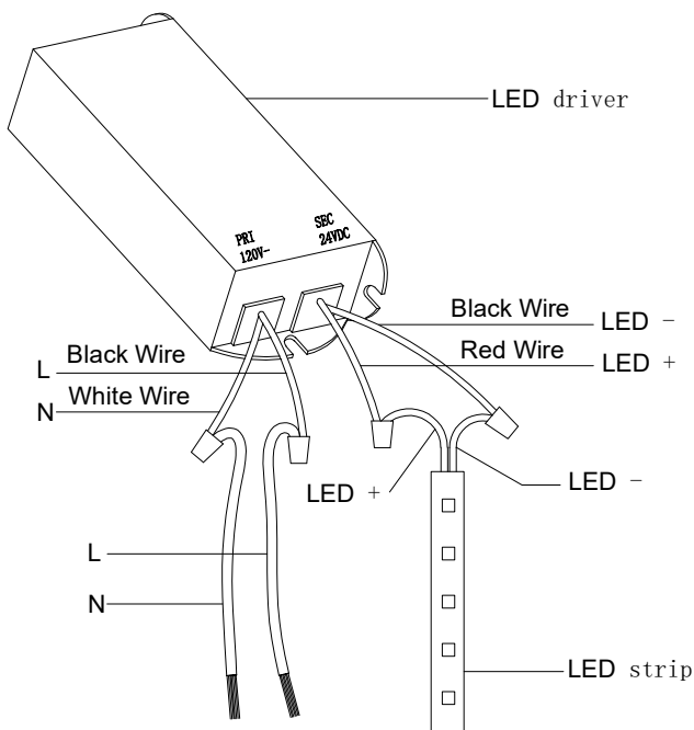
Wire connecting view
