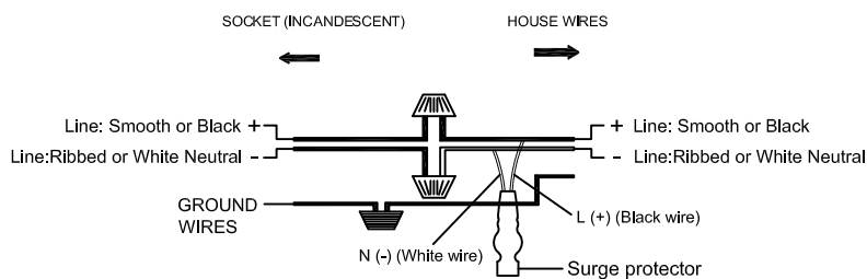
Wiring Diagram
