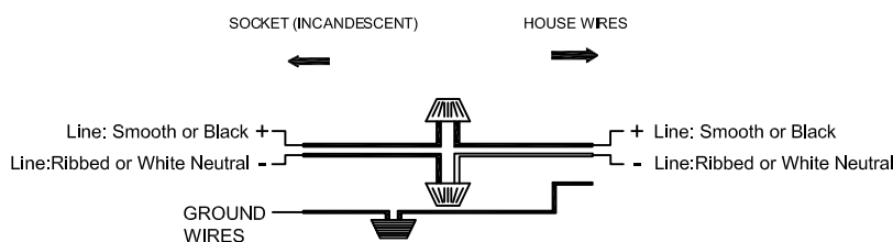
Wiring Diagram
