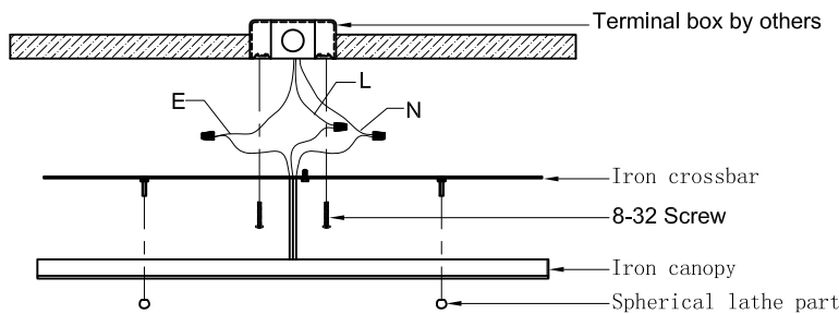
Wiring Diagram
