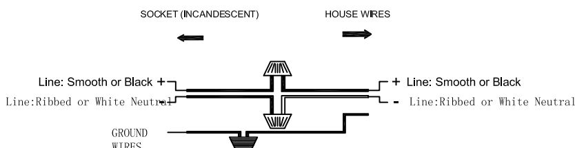
Wiring Diagram
