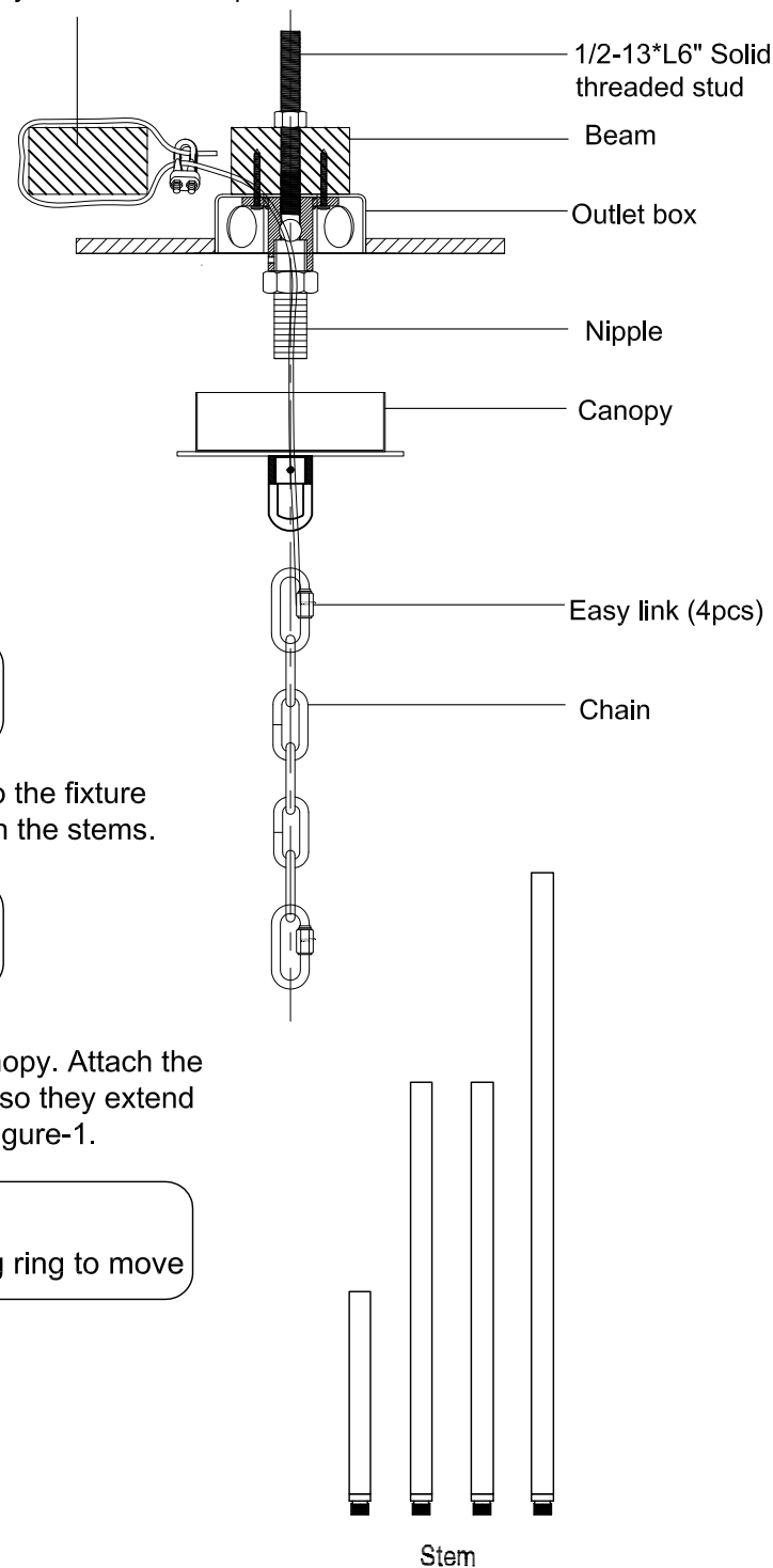
Safety cable fixed to separate beam
