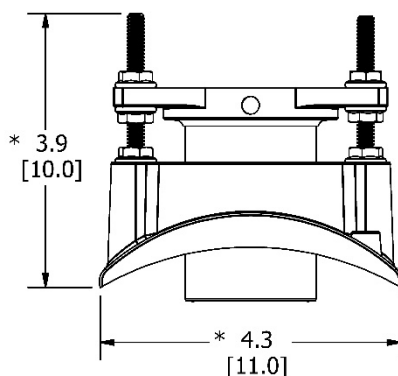
SADDLE – FRONT VIEW * In./cm
