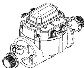
BSPP Meter (1/2 in. to 2 in.) Shown with Display Mount Cover Plate and Display
