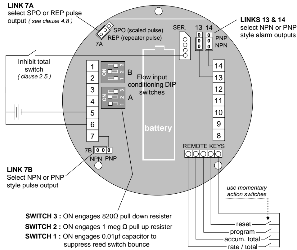
Terminal layout - links & remote switch inputs
