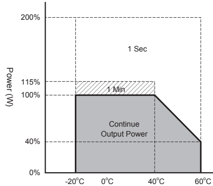
Temperature (°C) ISW-3000~4000 Power / Temperature Curve
