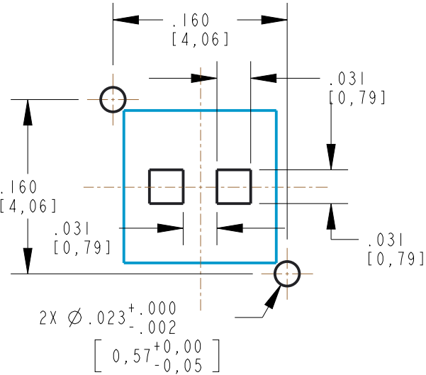
SINGLE COLOR 0603 W/ LENS 598-8EX10-107F LAYOUT
