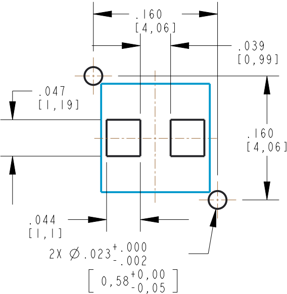
SINGLE COLOR 0805 598-81XX-107F LAYOUT
