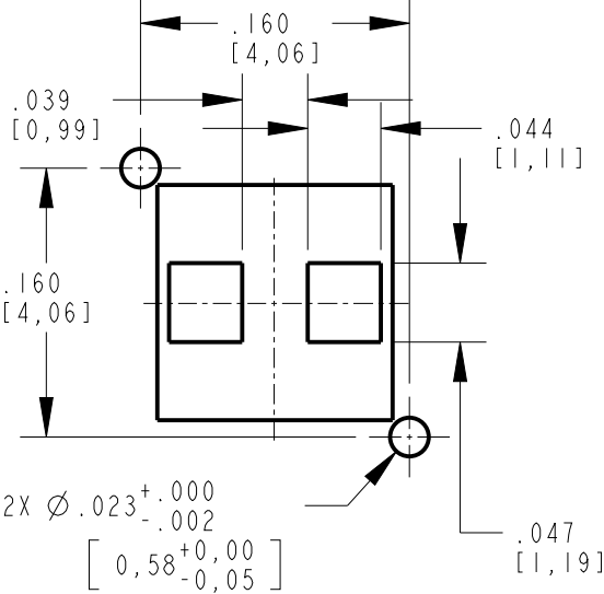
SINGLE COLOR 0805 598-81XX-107F LAYOUT
