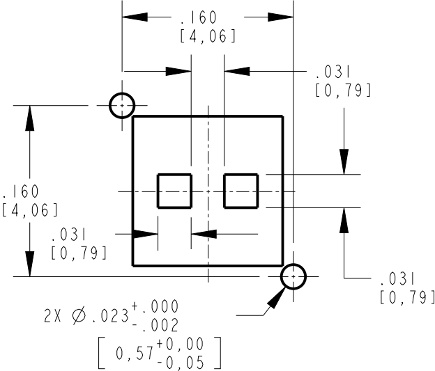
SINGLE COLOR 0603 W/ LENS 598-8EX10-107F LAYOUT
