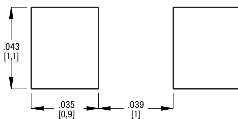
LED SCHEMATIC
