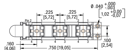
Bi-Color LED & Tri-Color LED Scale 6.000
