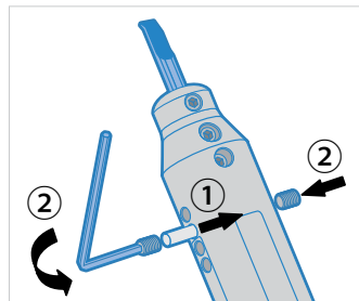
Fig. 1 How to Use Adjustment Pin
