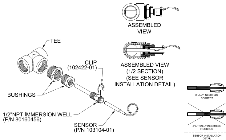
Figure 3-5: Recommended "Immersion" Type Header Sensor installation Detail
