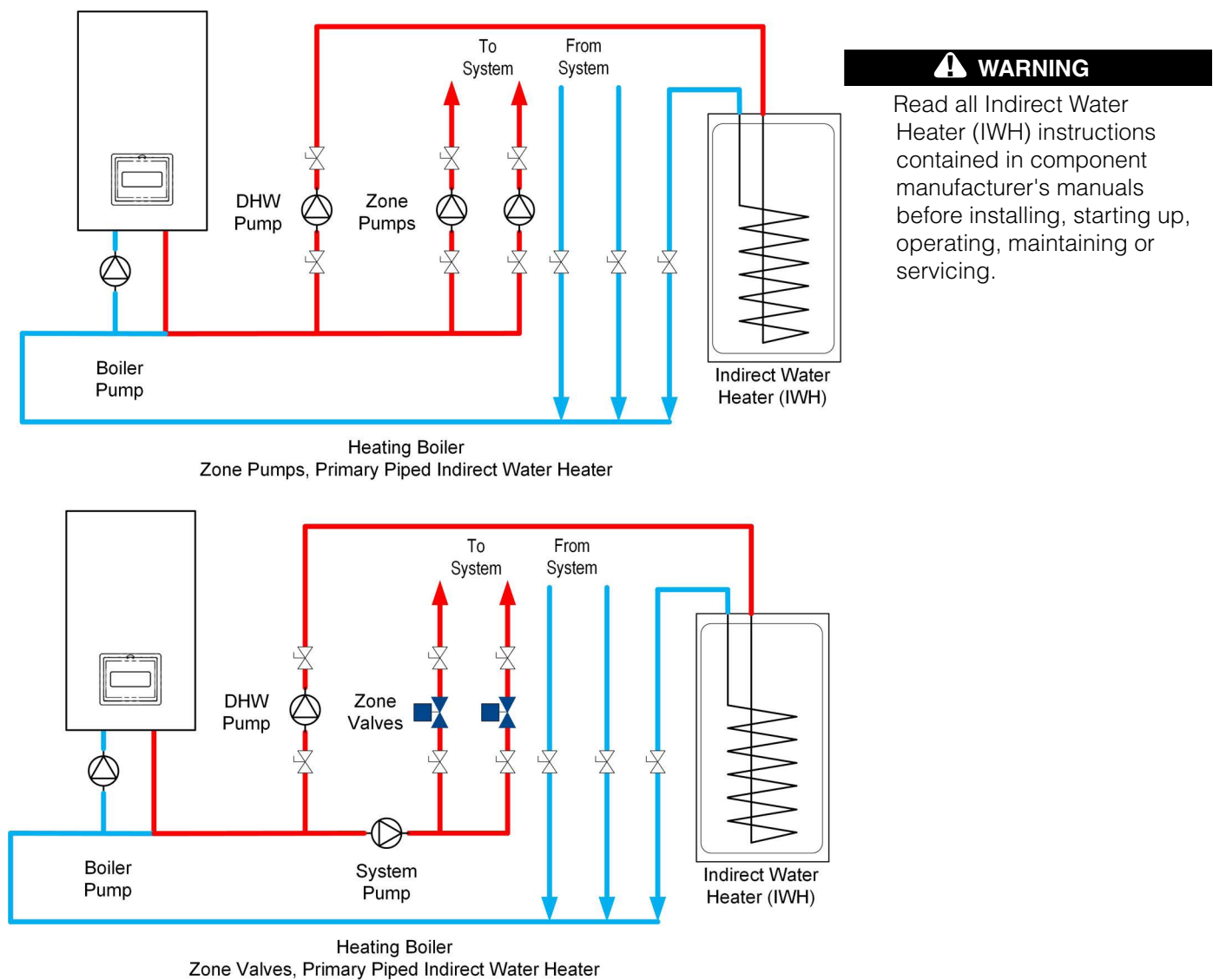
Figure 5-8: Example Pump Arrangements, Heating boiler, Primary Piped Indirect Water Heater (IWH)
