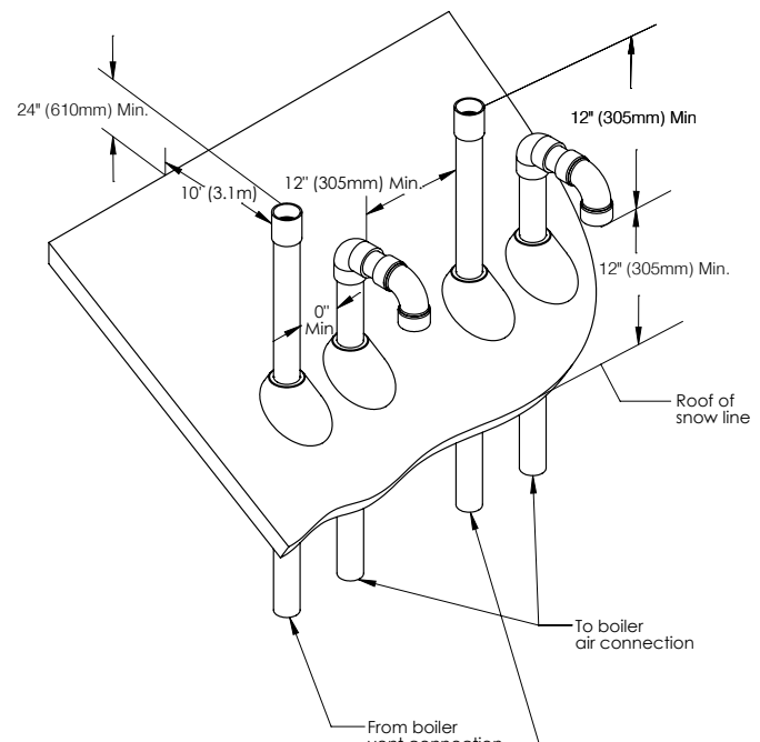
Figure 3-1: Multiple Boiler Terminations
