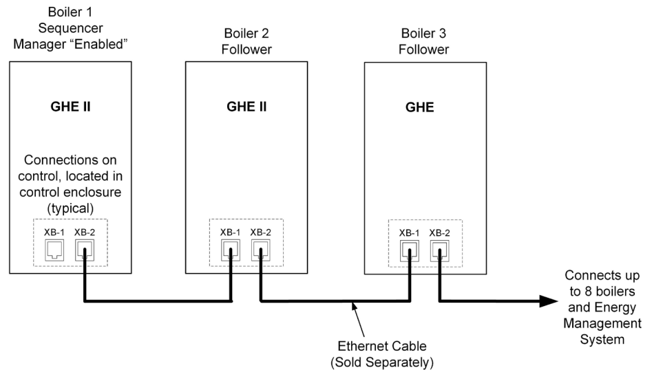
Figure 3-8: Boiler-to-Boiler Communication Network
