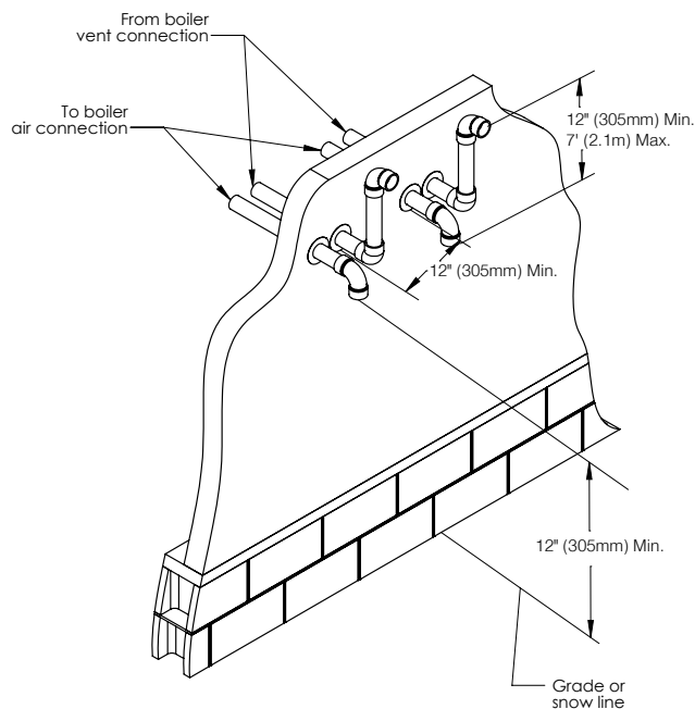
Figure 3-1: Multiple Boiler Terminations
