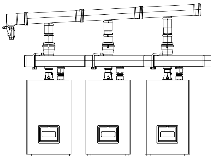
Figure 3-10: GHE II Heating Boiler Common Venting (Three shown, typical for 2 to 4)
