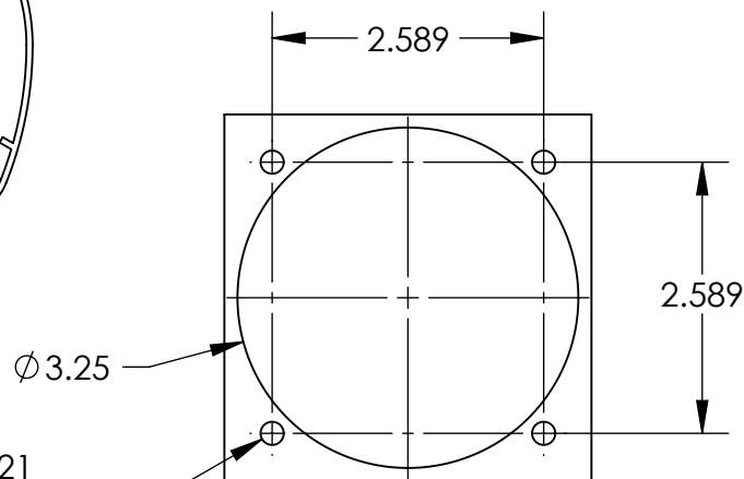
ENTRY HOLE PATTERN
