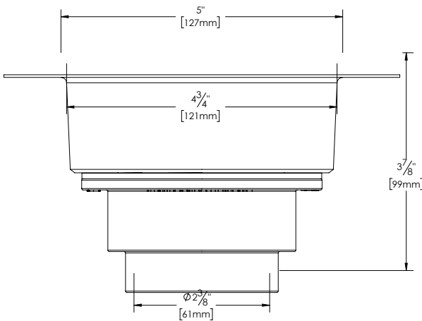
Fine Thread Brass Tailpiece Supplied with ID357 only .
