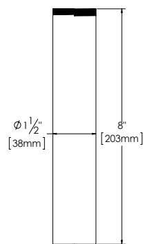
Fine Thread Brass Tailpiece Supplied with ID357 only .
