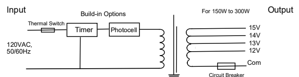
Wiring Diagram
