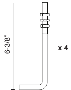
Anchor Bolt
