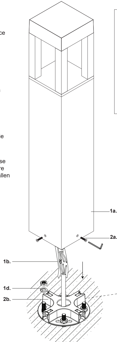
Anchor Bolt
