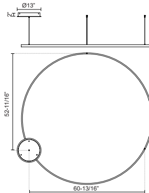
Side Canopy Option
