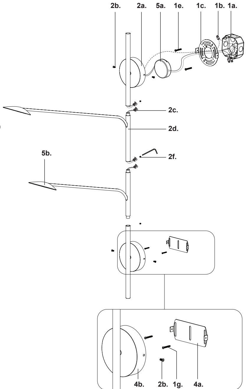
Illustration 1: Ideal distance of center of non-power mounting plate to center of mounting plate is 24-1/8".
