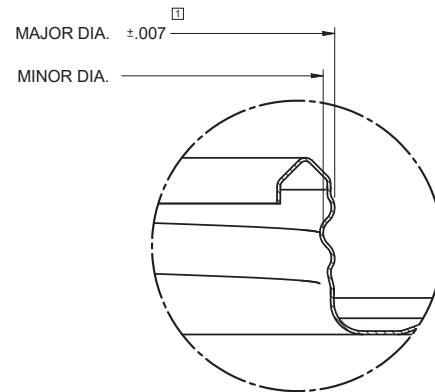
THREAD DETAIL
