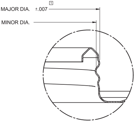
THREAD DETAIL
