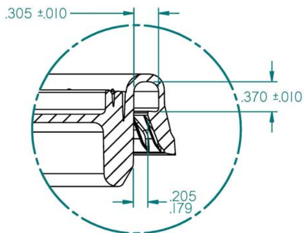
DETAIL B - GASKET CHANNEL SCALE: 1:1
