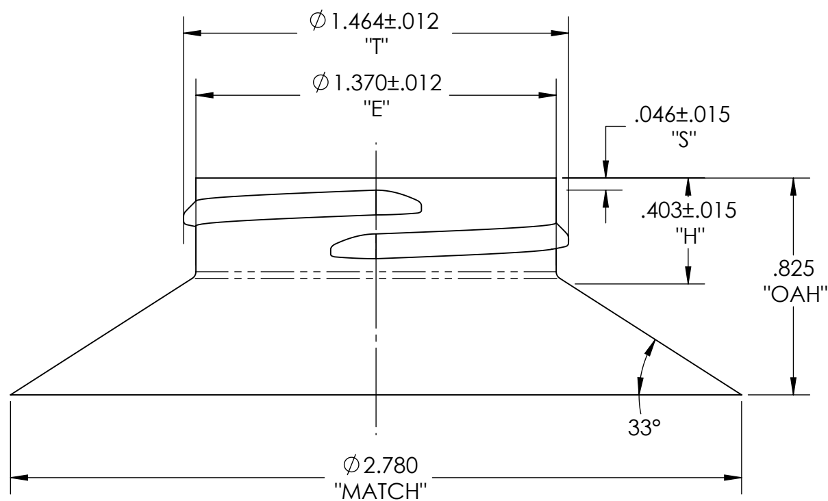
ALTERNATE 38mm NECK FINISH PER SPI STANDARDS
