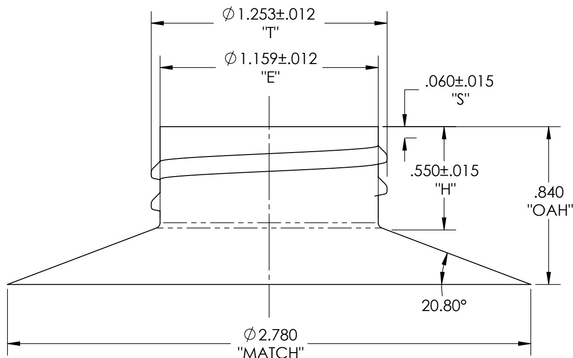
ALTERNATE 33mm NECK FINISH CUSTOM - PER CUSTOMER SAMPLE
