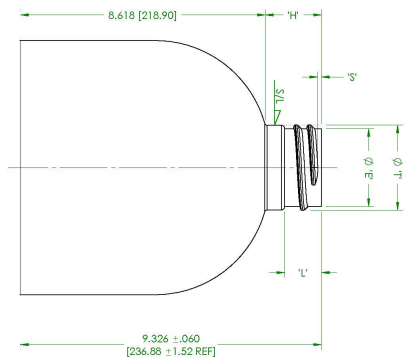
ALT NECK FINISH M28 SP410
