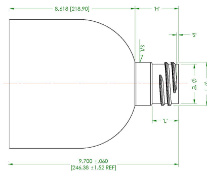
ALT NECK FINISH M28 SP415
