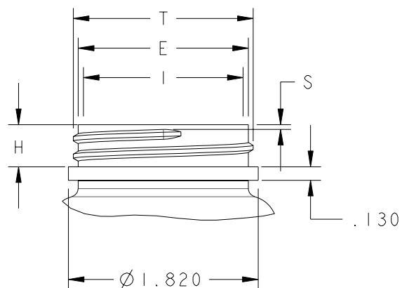
DETAIL A SCALE 5/4
