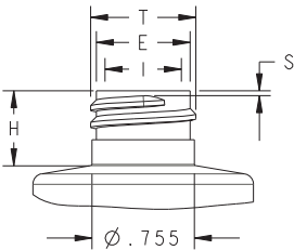
DETAIL A SCALE 3/2
