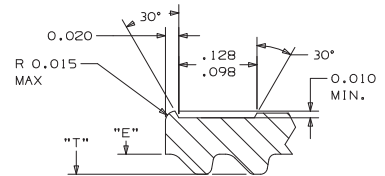
UNDERCUT DETAIL
