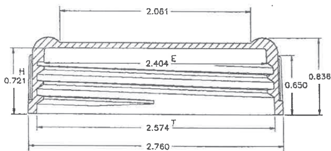
CAP SECTION
