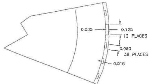
RIB DETAIL
