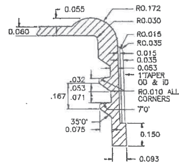
THREAD DETAIL
