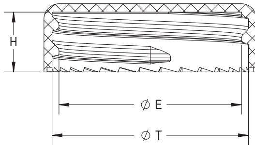
SECTION G-G
