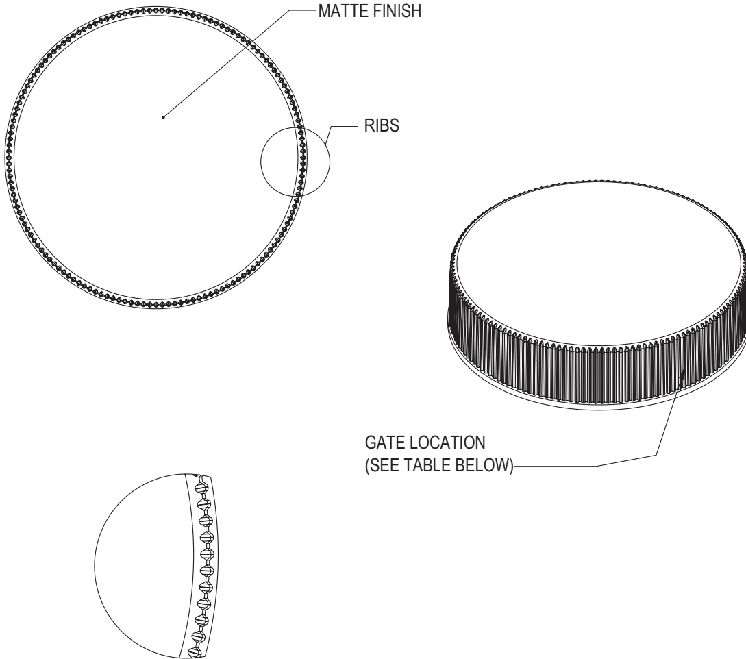
148 EQUALLY SPACED RIBS DETAIL RIBS SCALE 4 : 1
