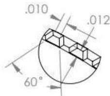
120 KNURLS DETAIL B SCALE 10 : 1
