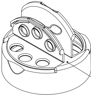
300 / POUR OPTION PART WEIGHT: 9.52 grams SIFT DISPENSING AREA: 0.212 IN 2
