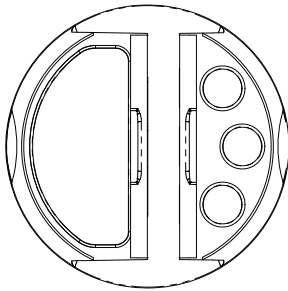
300 / POUR OPTION PART WEIGHT: 9.52 grams SIFT DISPENSING AREA: 0.212 IN 2
