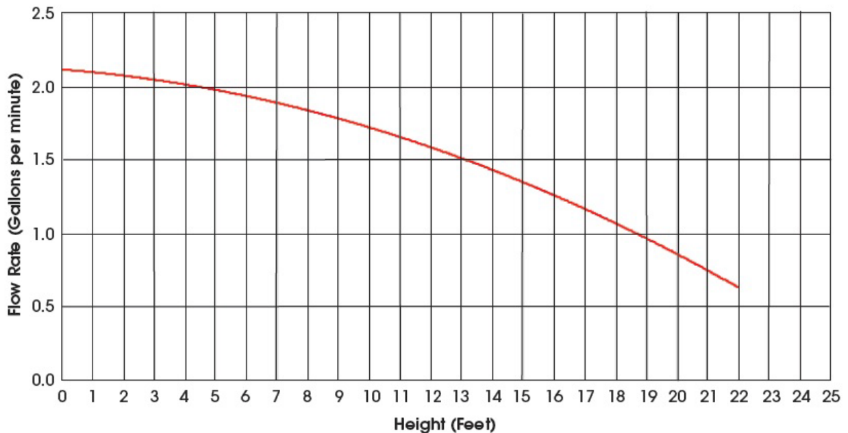
CP-22LP Pump Performance Curve
