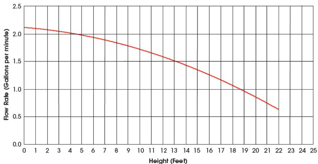
ULTRACP-22 Pump Performance Curve
