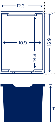
Standard Jumbo Tray
