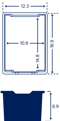
Standard Extra Deep Tray
