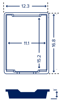
Standard Shallow Tray
