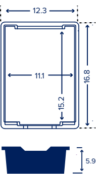
Standard Deep Tray
