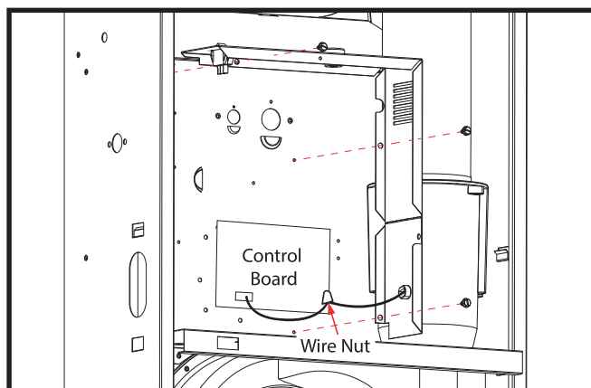
Figure 2. Control Box Installation
