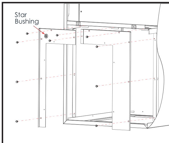
Figure 2. Coil Close Off Panels
