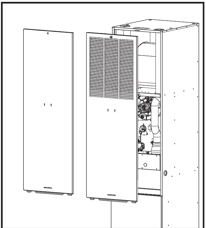
Figure 7. Upper Door
