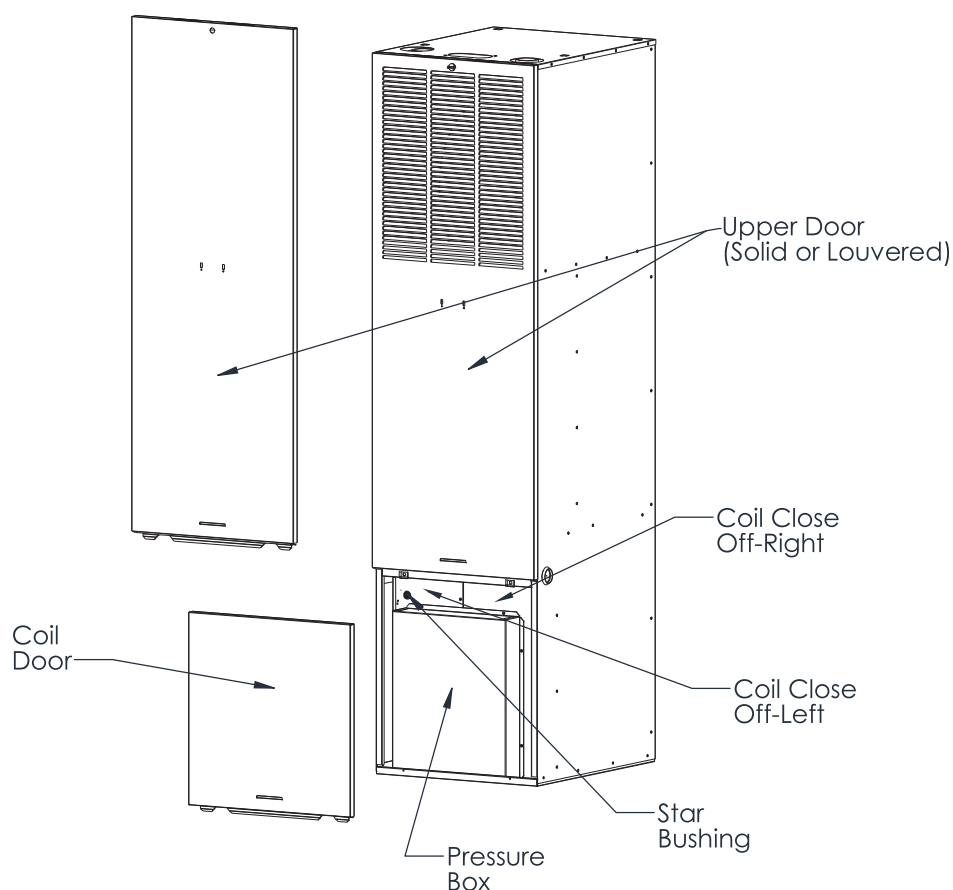
Figure 1. MG2S "B" Cabinet Part List
