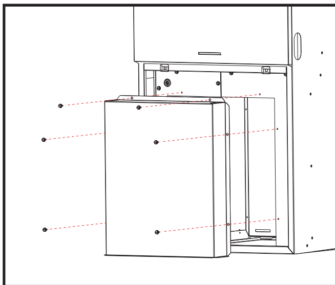
Figure 5. Pressure Box
