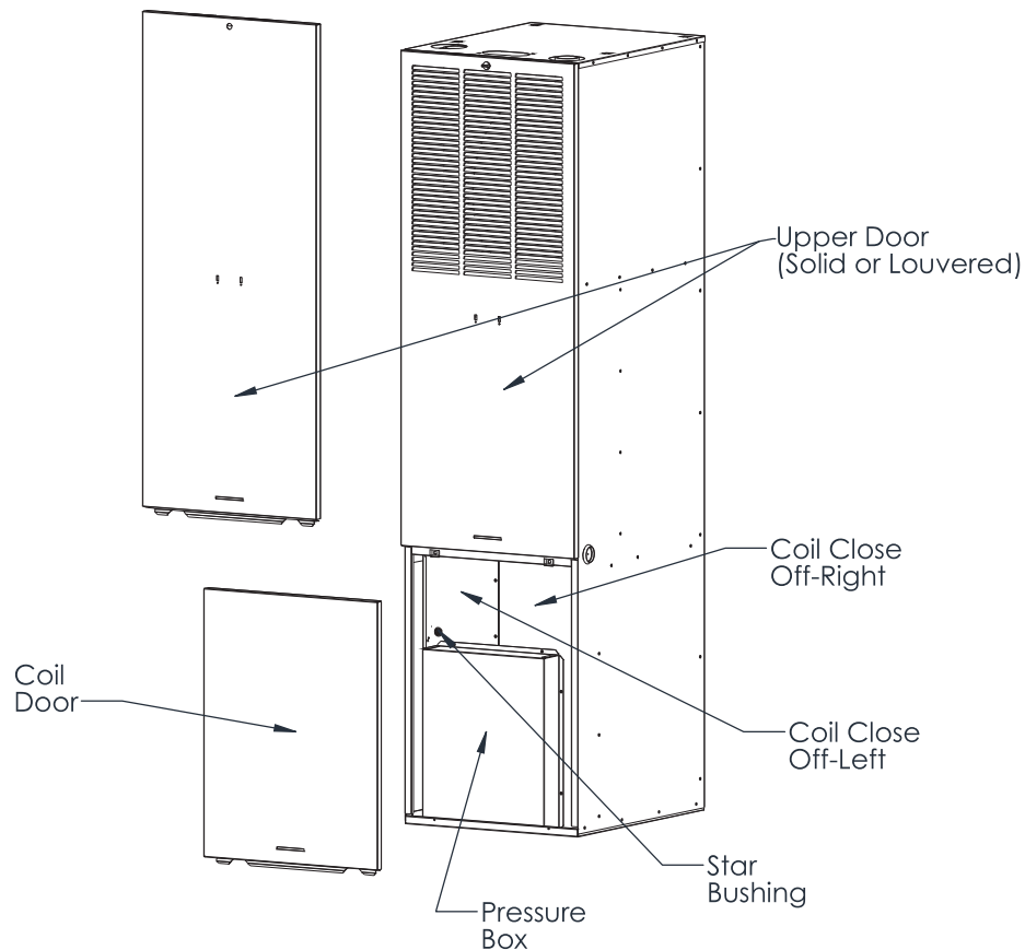
Figure 1. MG2R "C" Cabinet Part List
