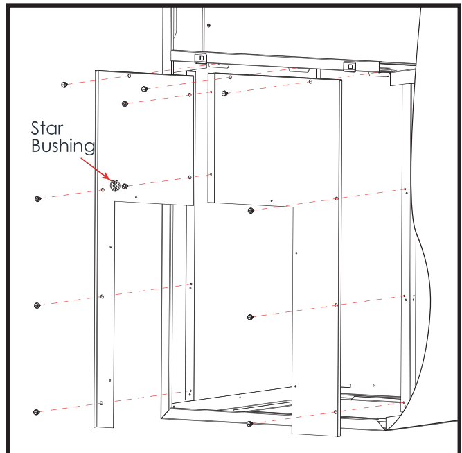
Figure 2. Coil Close Off Panels
