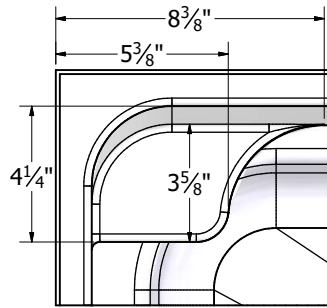
Shelf Detail
