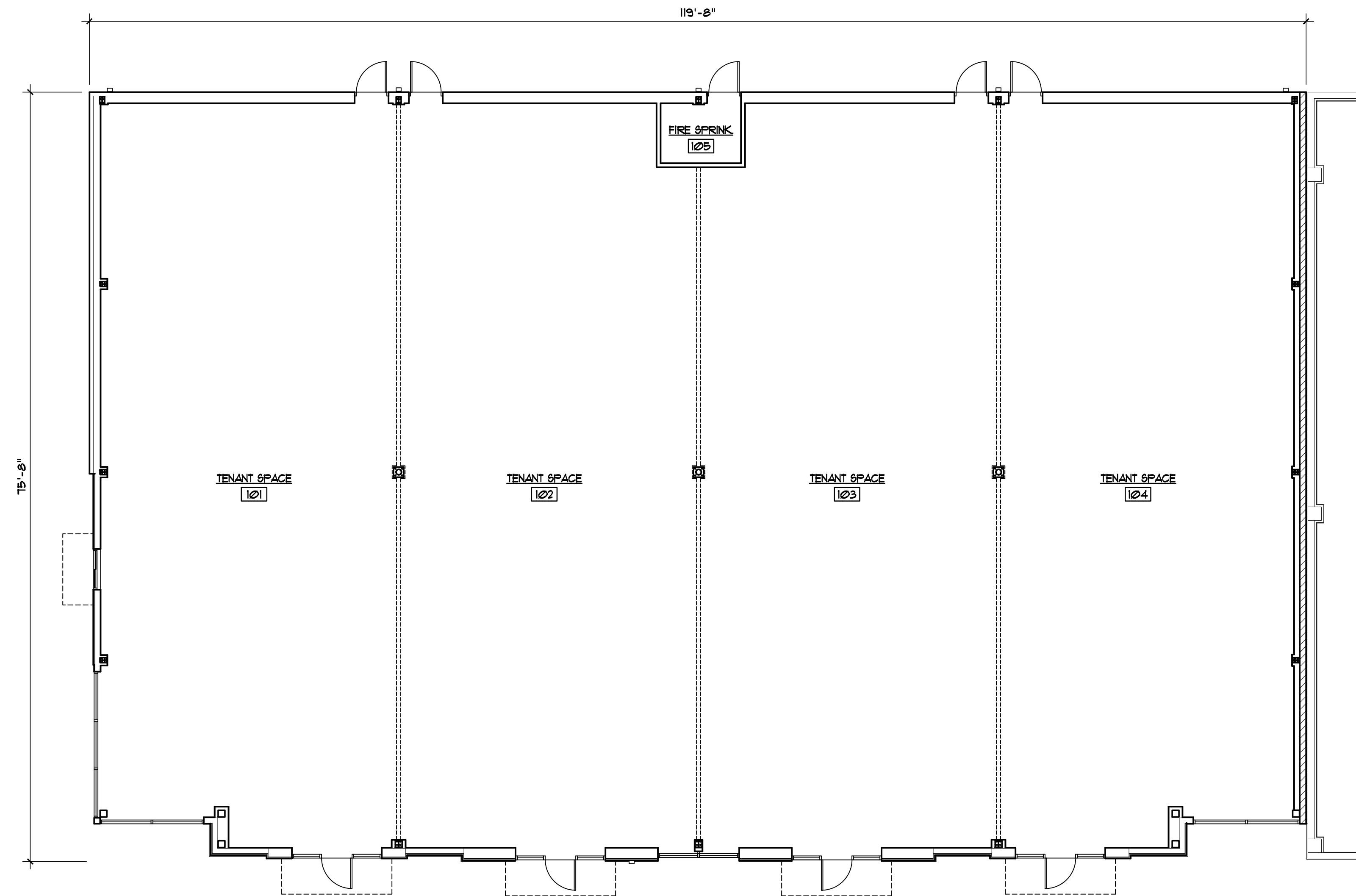
FLOOR PLAN 1/8" = 1'-0" AREA: 8,930 S.F.
