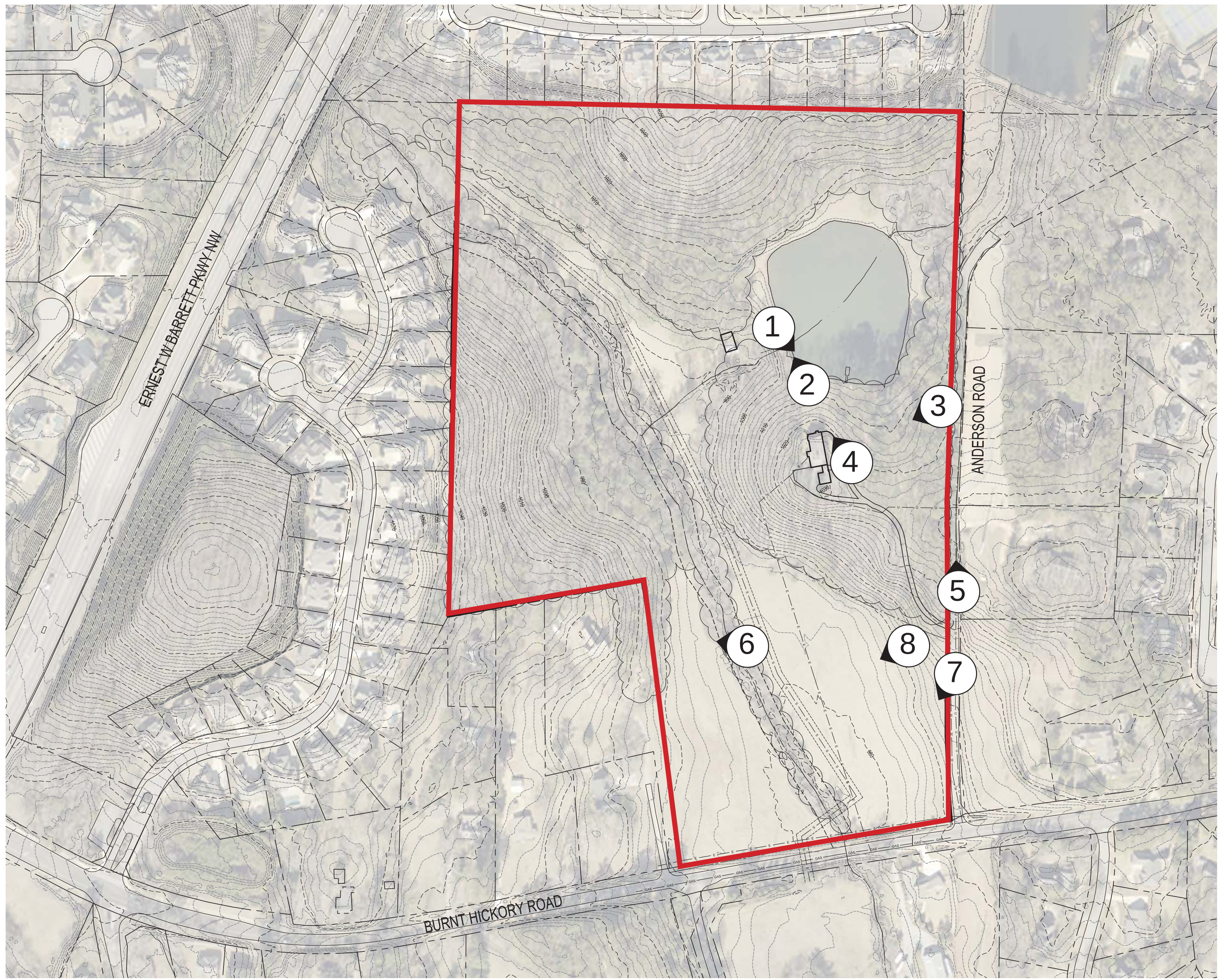
EXISTING SURVEY WITH AERIAL MAP OVERLAY
