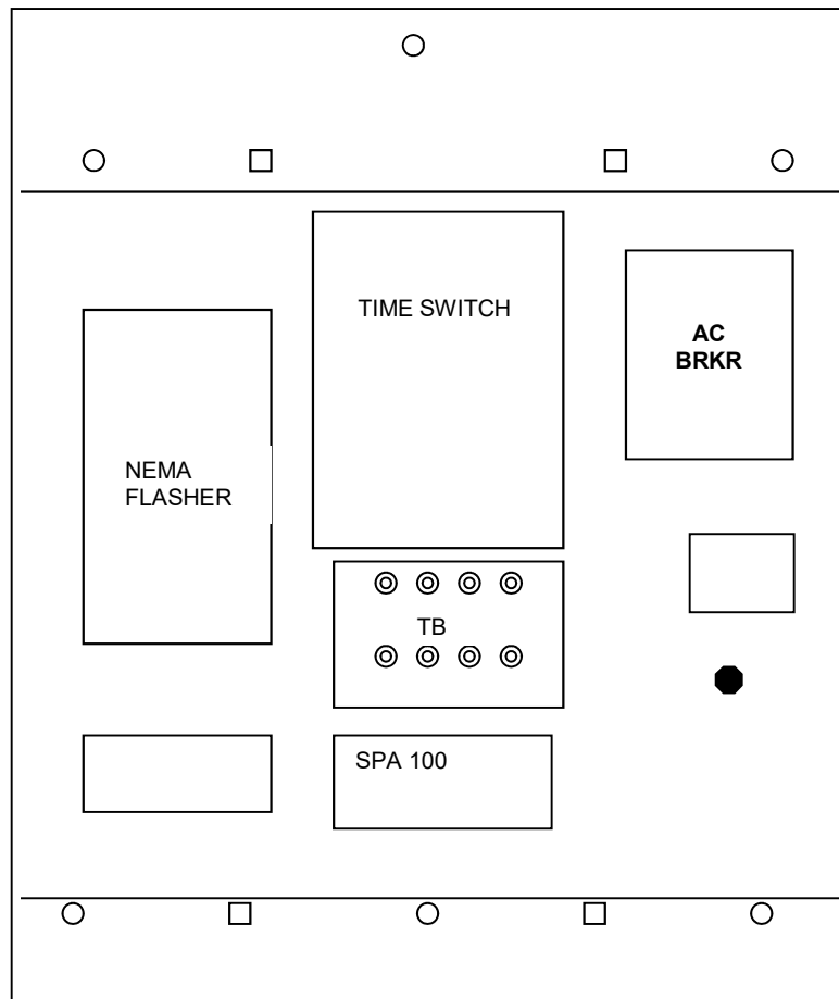
Figure 925-14—Typical Flashing Cabinet Layout
