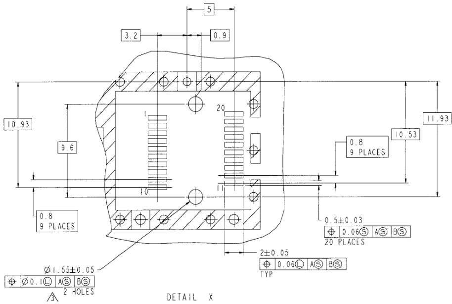
DETAIL X
